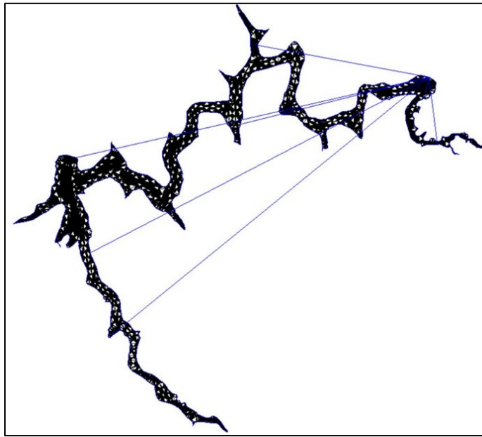
Figure 15. 2023 Beech Fork Lake bathymetry survey TIN model.
