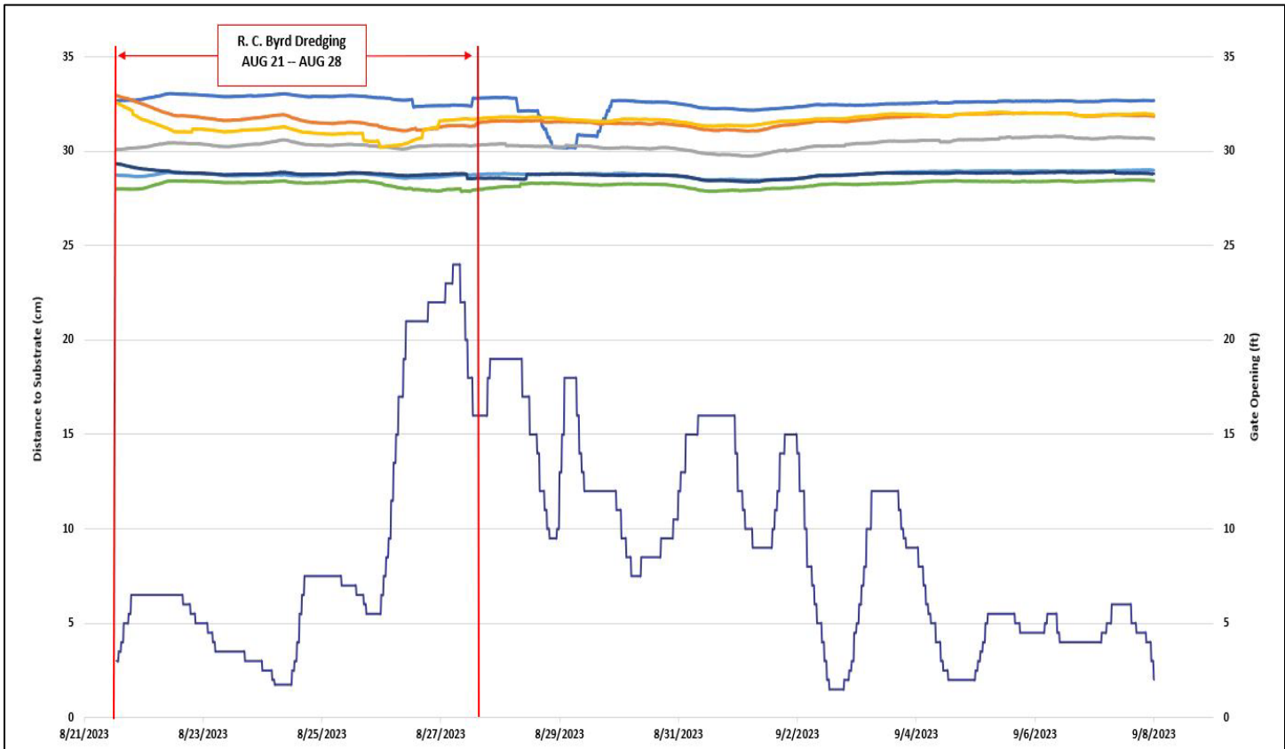
Figure 10. WIZARD transducer results for August deployment smoothed to account for daily temperature interference.
