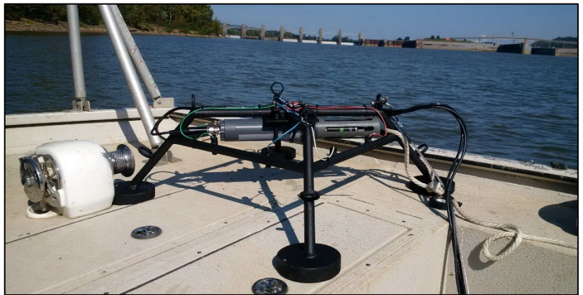
Figure 8. The WIZARD measures conditions in the actual substrate and the water column.
