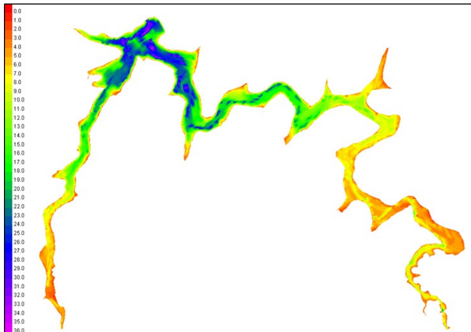
Figure 16. 2023 Beech Fork Lake bathymetry survey depth raster. Depths in feet.
